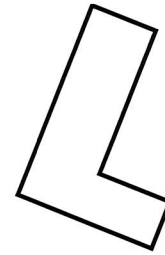
Figure 12. Irregular hexagon.
